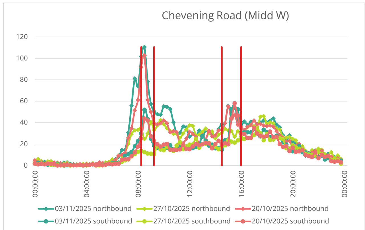
Figure 9 - ATC directional flow graph for Chevening Road (Midd W) (Site 9)
