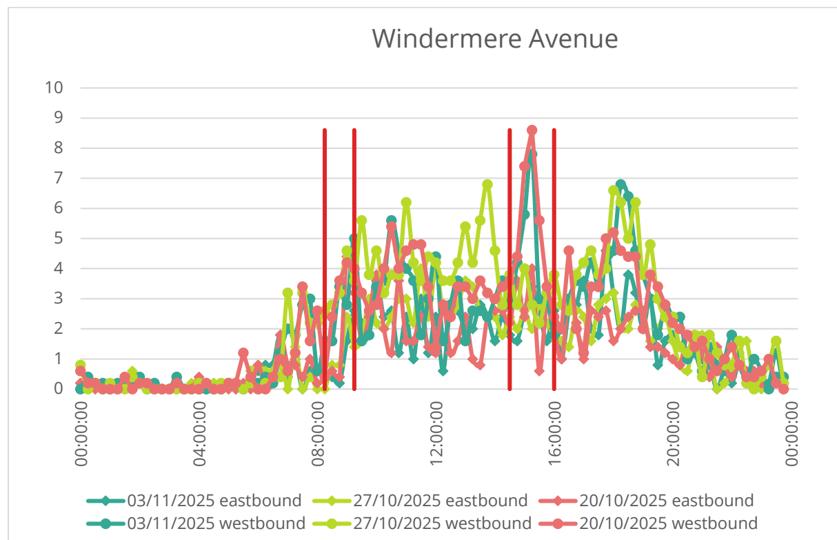
Figure 21 - ATC directional flow graph for Windermere Avenue (Site 22)
