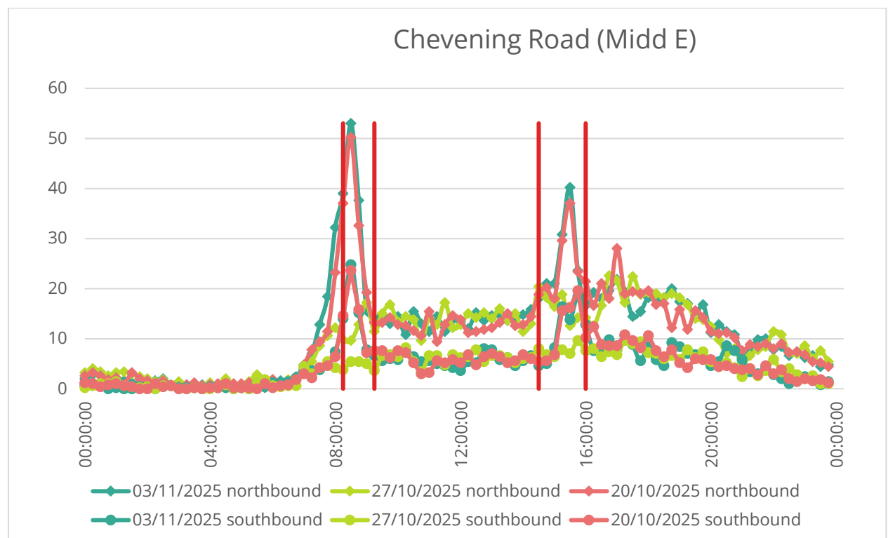
Figure 10 - ATC directional flow graph for Chevening Road (Midd E) (Site 10)
