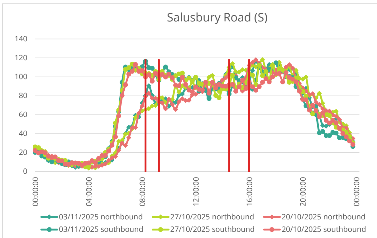
Figure 16 - ATC directional flow graph for Salusbury Road (S) (Site 16)
