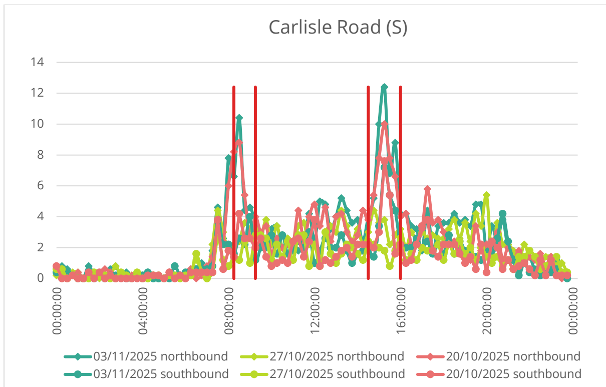
Figure 19 - ATC directional flow graph for Carlisle Road (S) (Site 20)
