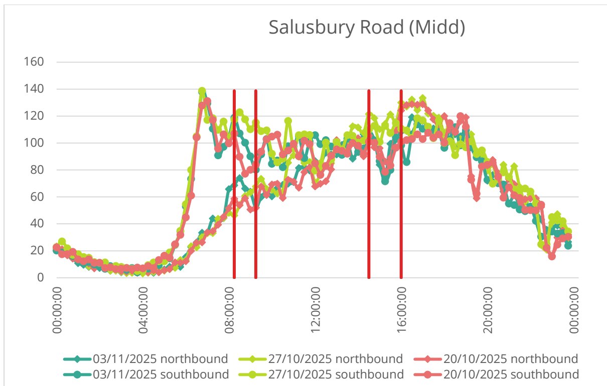
Figure 15 - ATC directional flow graph for Salusbury Road (Midd) (Site 15)
