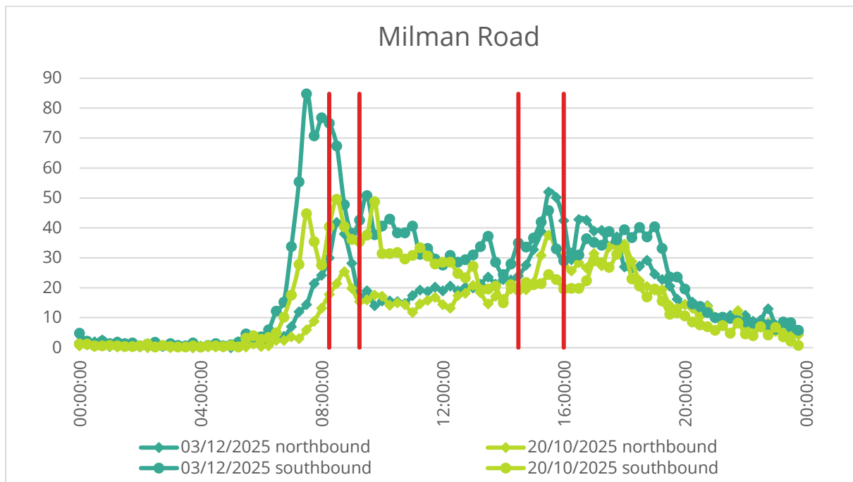
Figure 33 - ATC directional flow graph for Milman Road (Site 35)
