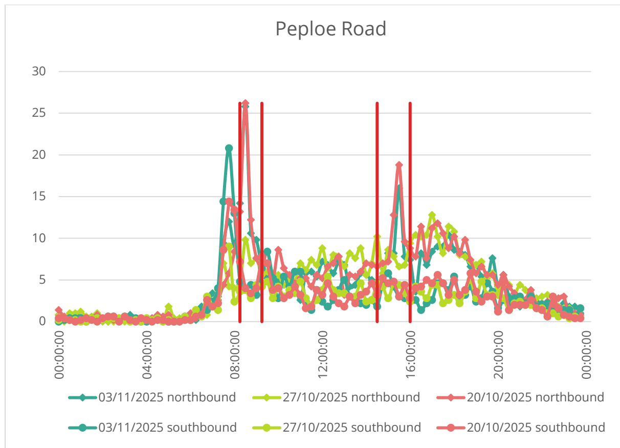
Figure 35 - ATC directional flow graph for Peploe Road (Site 27)
