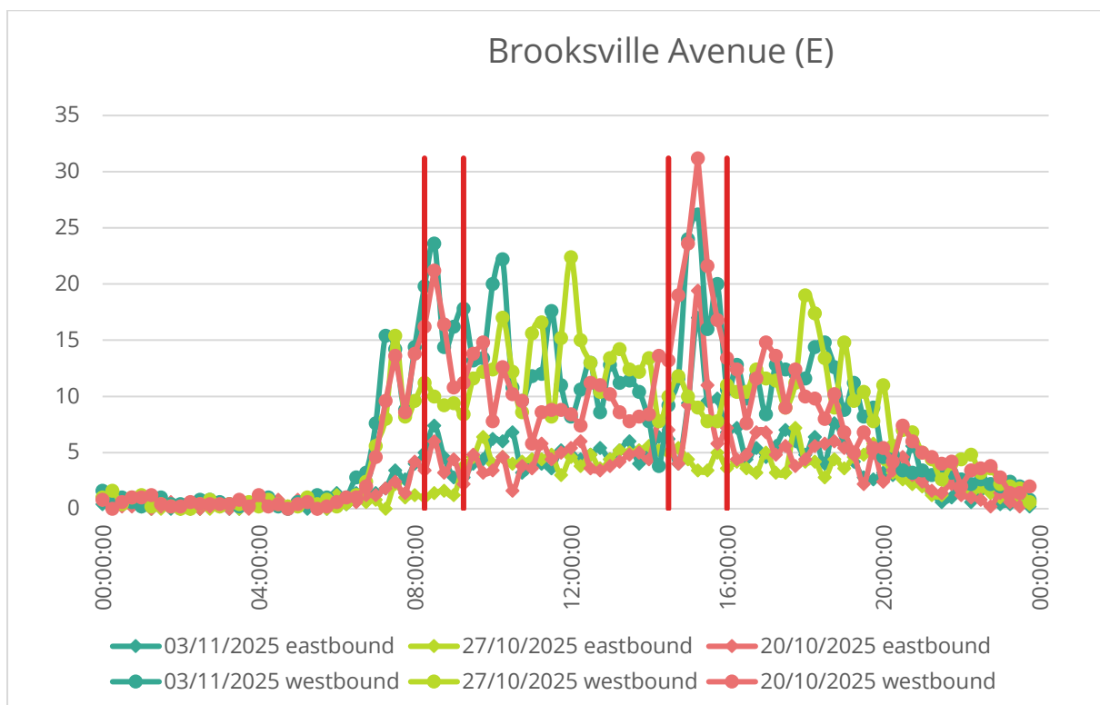
Figure 20 - ATC directional flow graph for Brooksville Avenue (E) (Site 21)
