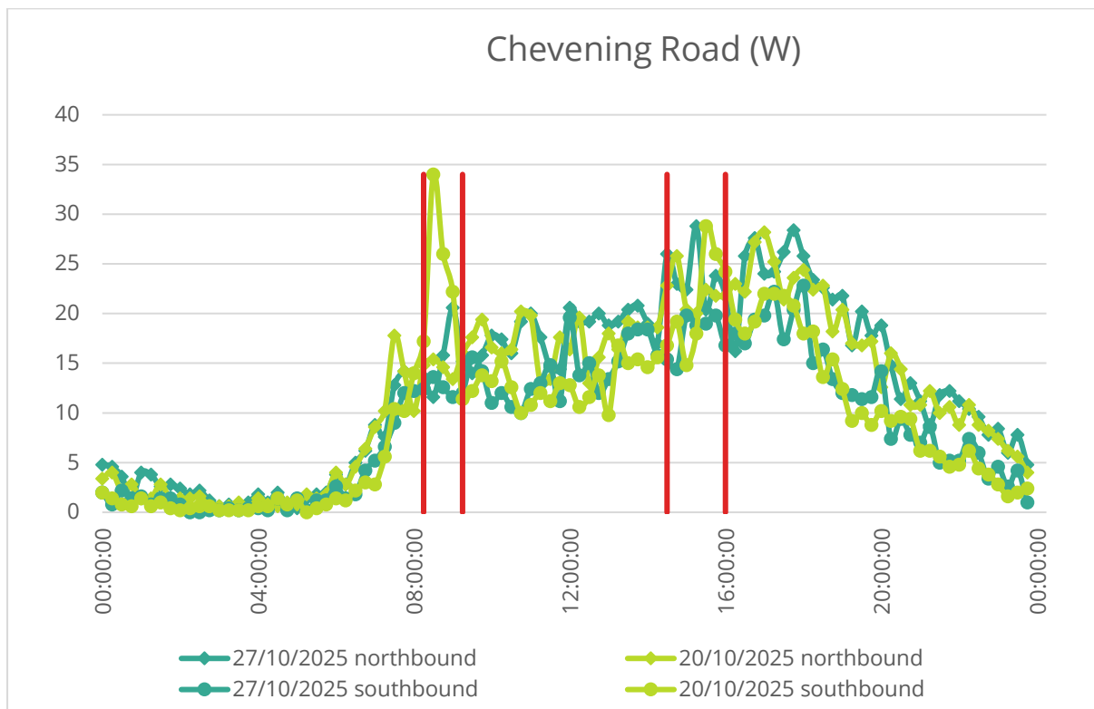
Figure 8 - ATC directional flow graph for Chevening Road (W) (Site 8)
