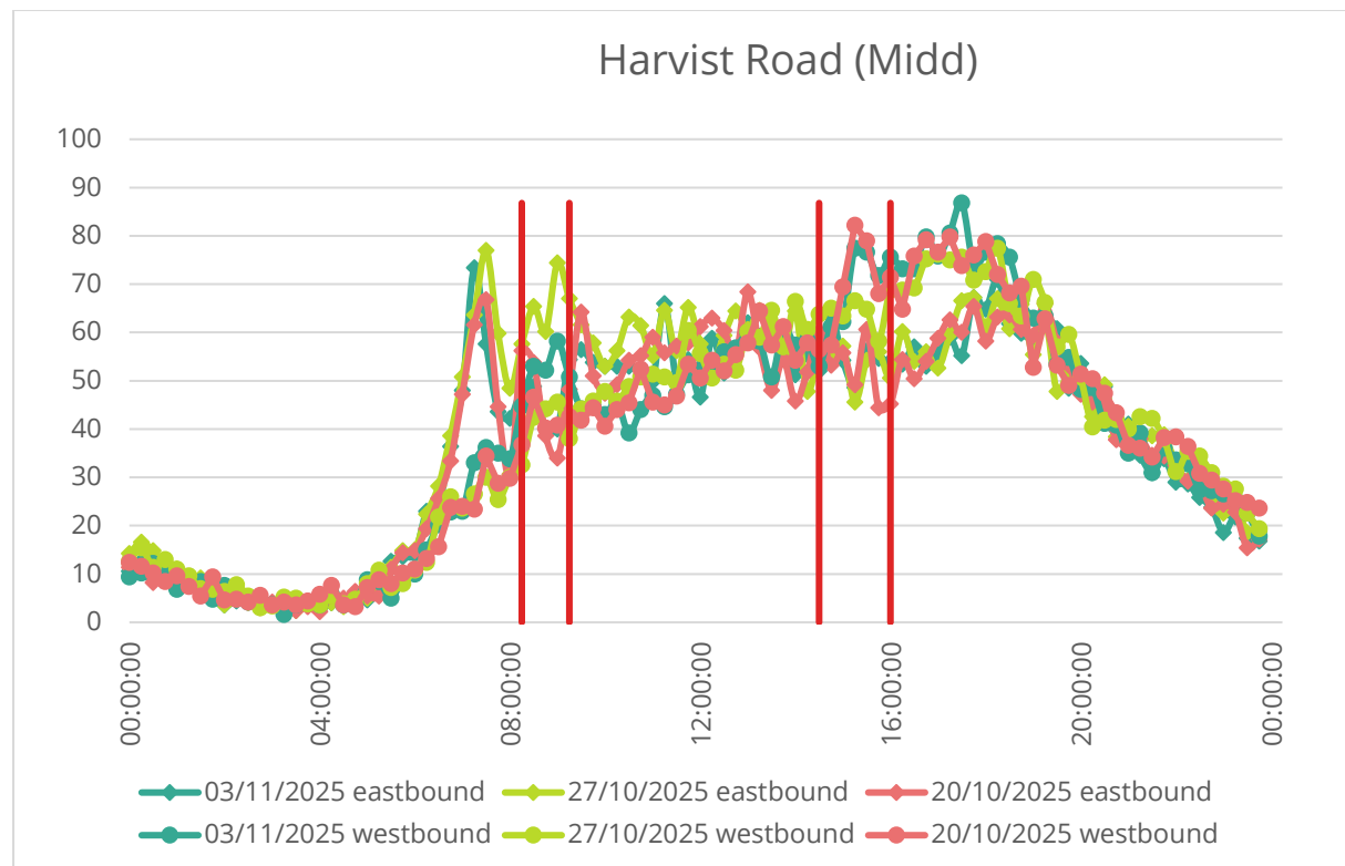
Figure 31 - ATC directional flow graph for Harvist Road (Midd) (Site 33)
