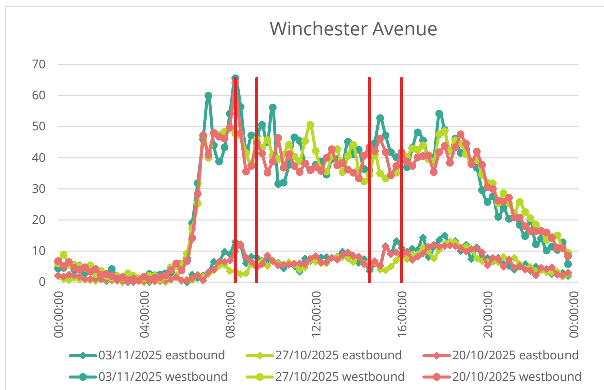
Figure 12 - ATC directional flow graph for Winchester Avenue (Site 12)
