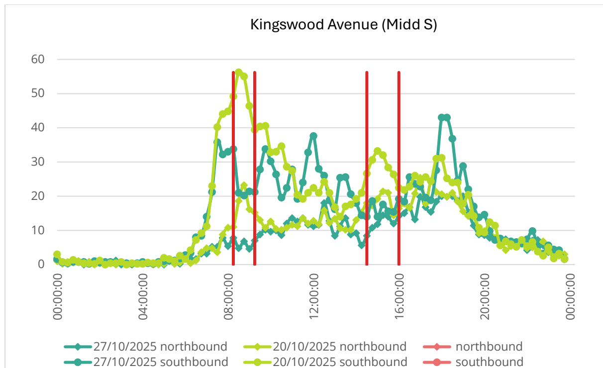
Figure 27 - ATC directional flow graph for Kingswood Avenue (Midd S) (Site 29)
