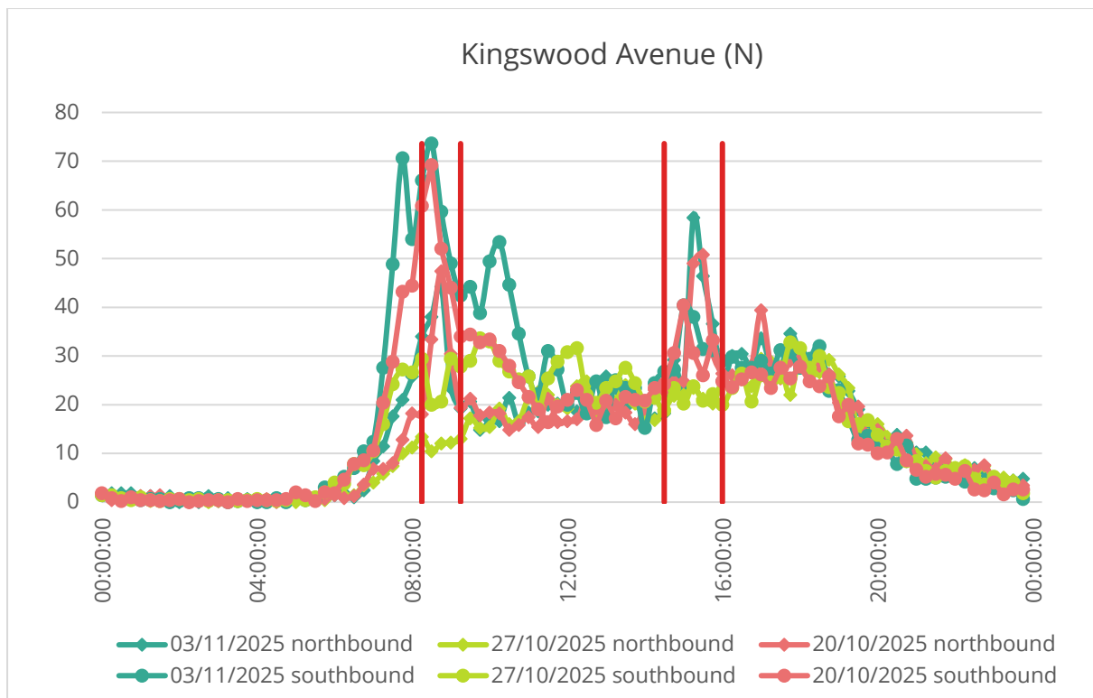
Figure 29 - ATC directional flow graph for Kingswood Avenue (N) (Site 31)
