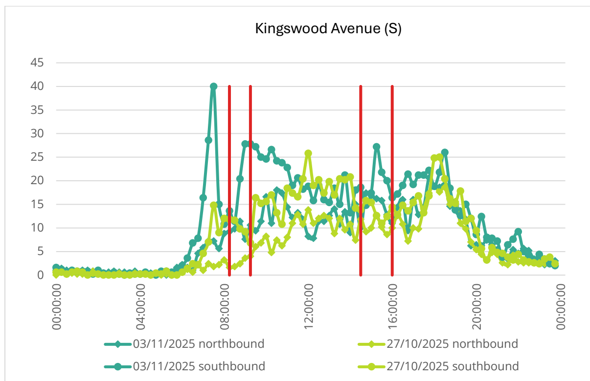
Figure 26 - ATC directional flow graph for Kingswood Avenue (S) (Site 28)
