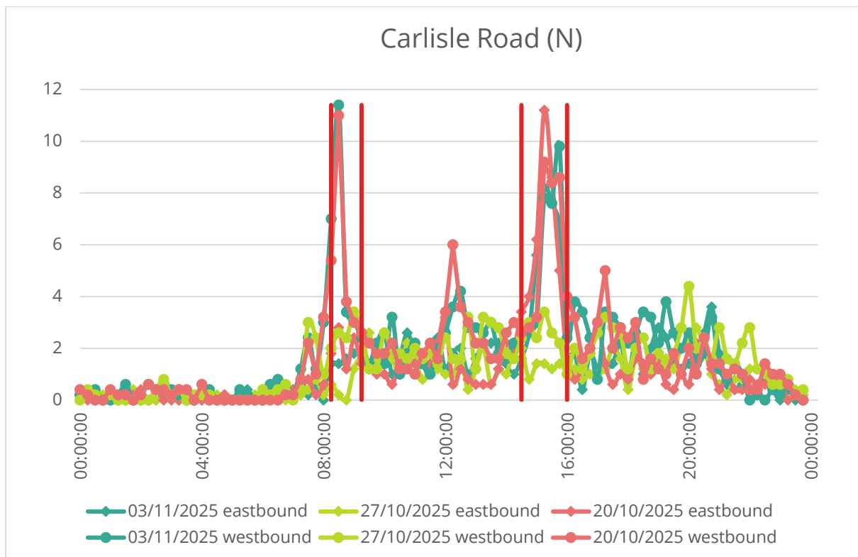
Figure 17 - ATC directional flow graph for Carlisle Road (N) (Site 17)
