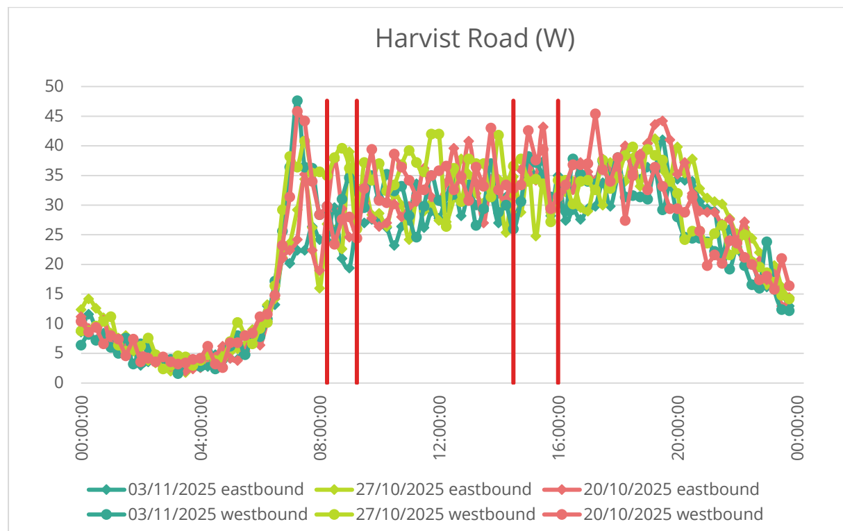
Figure 32 - ATC directional flow graph for Harvist Road (W) (Site 34)
