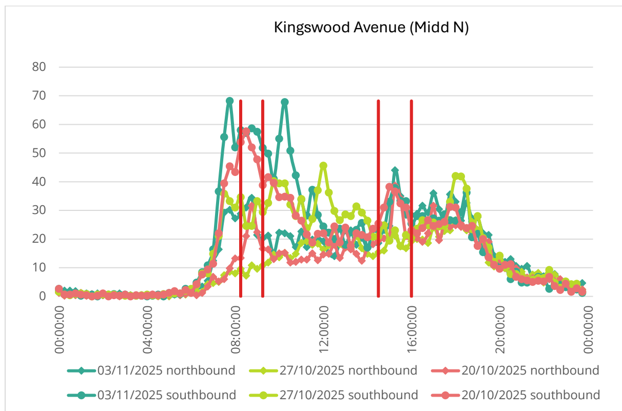
Figure 28 - ATC directional flow graph for Kingswood Avenue (Midd N) (Site 30)
