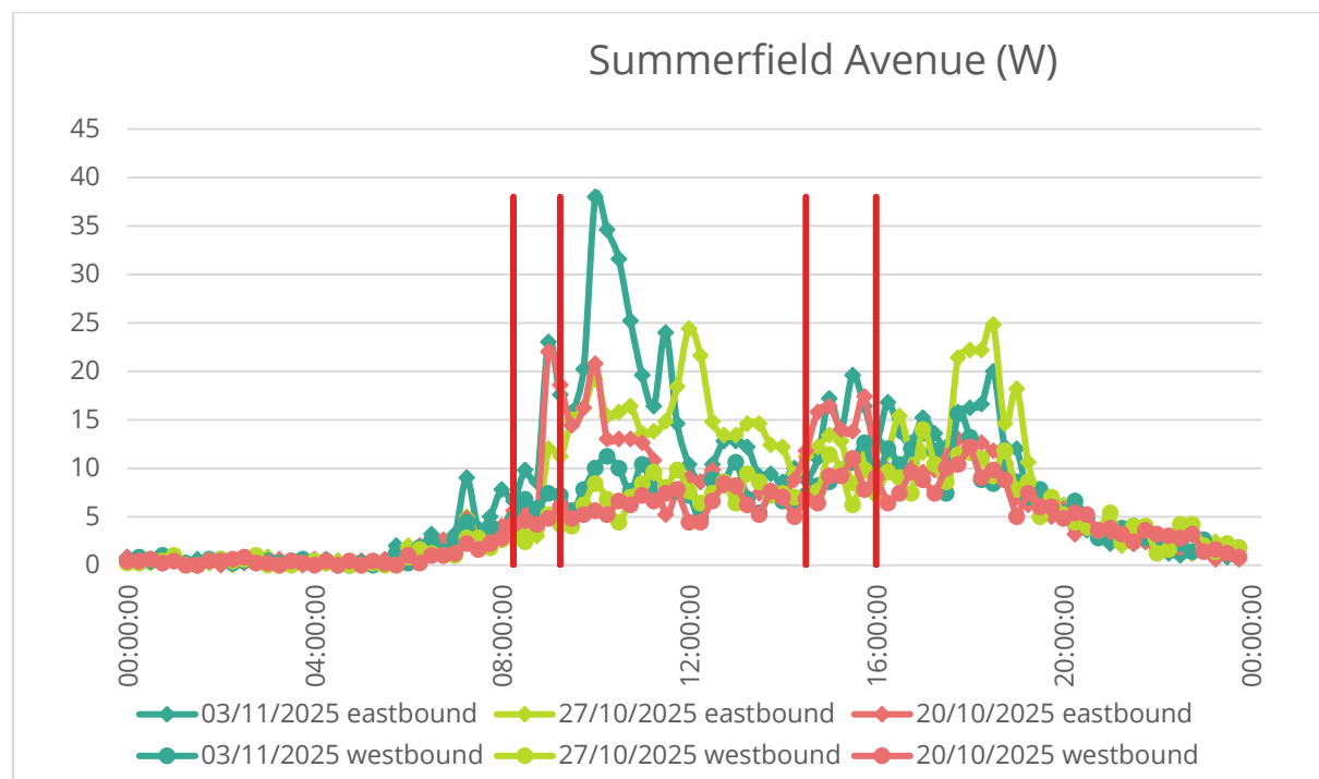
Figure 24 - ATC directional flow graph for Summerfield Avenue (W) (Site 25)
