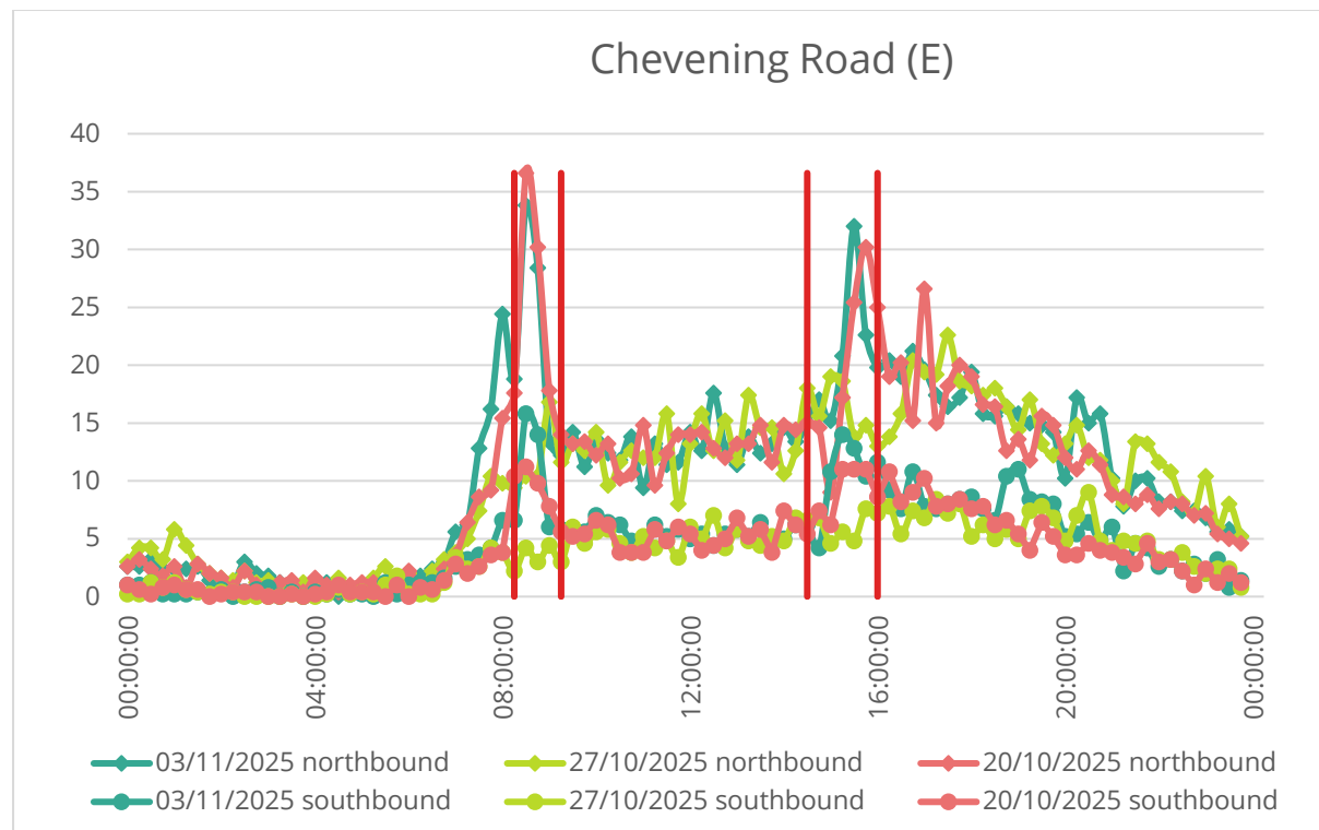
Figure 11 - ATC directional flow graph for Chevening Road (E) (Site 11)
