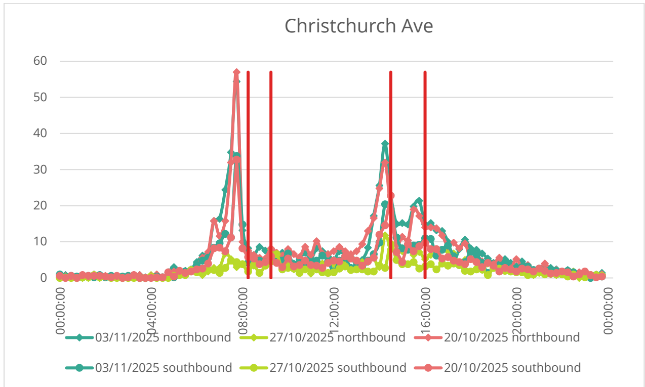
Figure 1 - ATC directional flow graph for Christchurch Avenue (Site 1)
