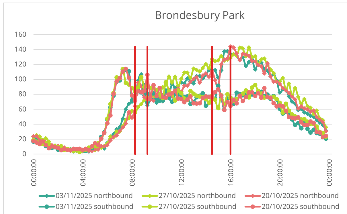
Figure 13 - ATC directional flow graph for Brondesbury Park (Site 13)
