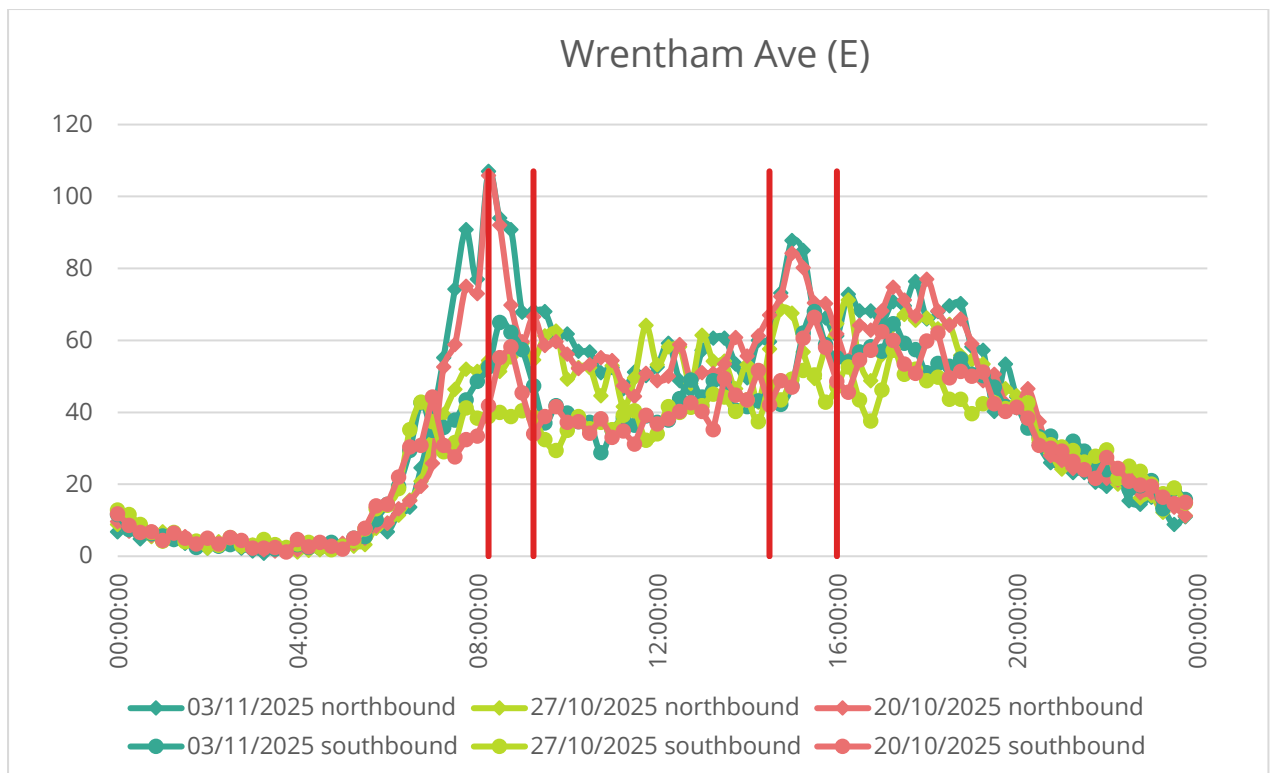
Figure 5 - ATC directional flow graph for Wrentham Ave (E) (Site 5)
