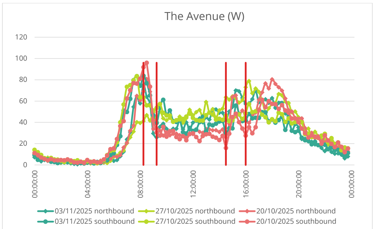
Figure 4 - ATC directional flow graph for The Avenue (E) (Site 3)
