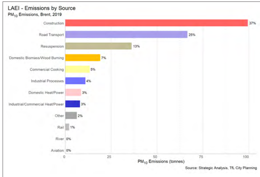
Figure 14: PM10 Emissions by Source (LAEI 2019)
